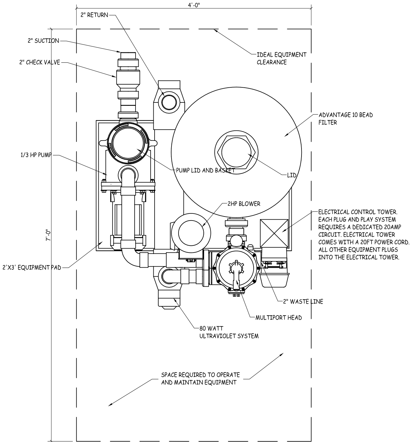
11 6K PLUG AND PLAY 1" = 1'-0" TYPICAL LAYOUT
