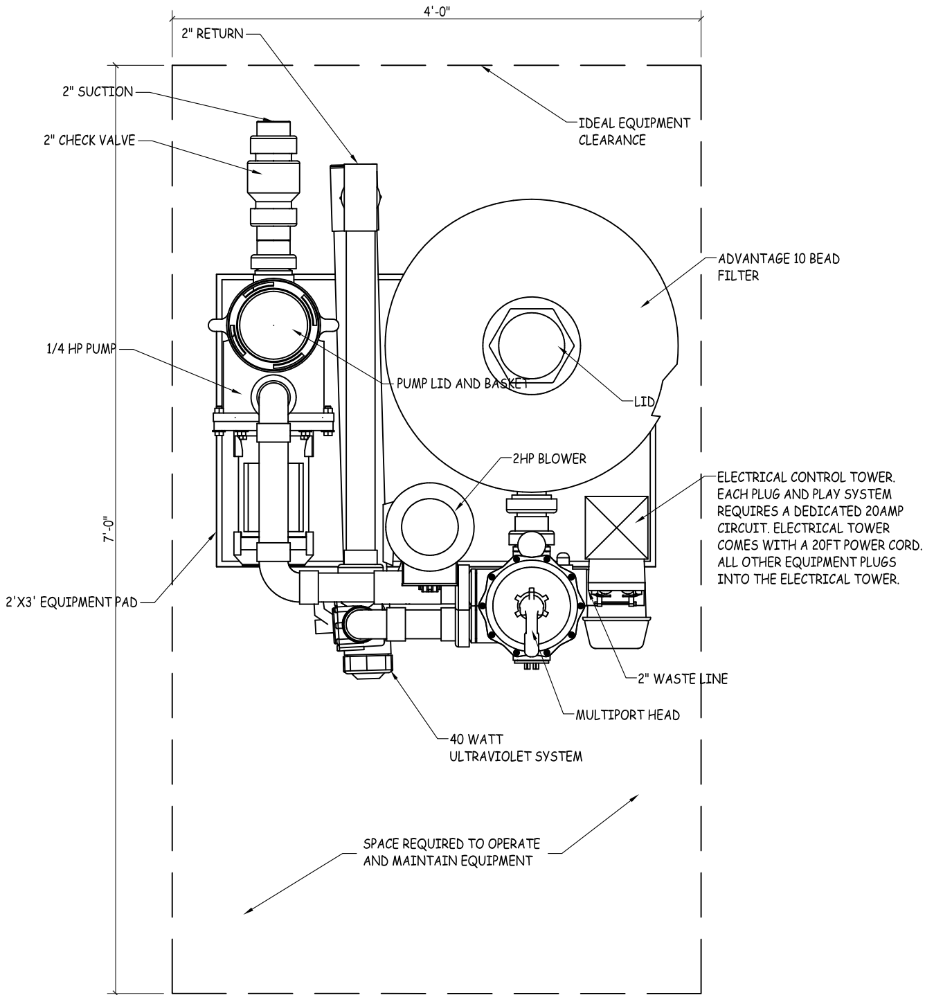
10 2K PLUG AND PLAY 1" = 1'-0" TYPICAL LAYOUT
